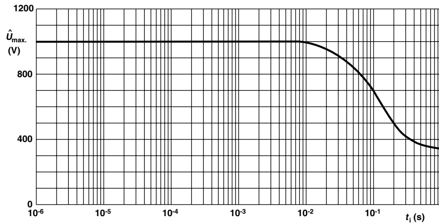
NFR25H Pulse on a regular basis; maximum permissible peak pulse voltage ( \hat{U}_{max.} ) as a function of pulse duration ( t_i )
