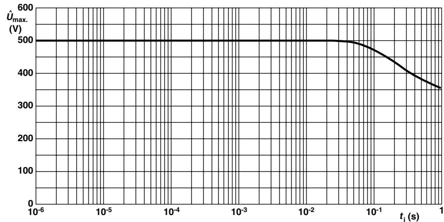
NFR25 Pulse on a regular basis; maximum permissible peak pulse voltage \hat{U}_{max.} as a function of pulse duration ( t_i )
