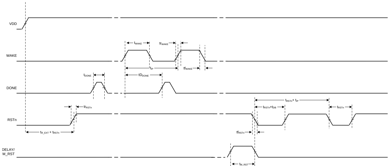
Figure 1. TPL5010 Timing
