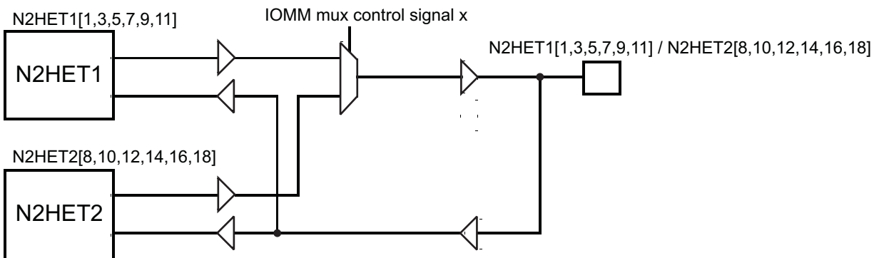
Figure 5-7. N2HET Monitoring
