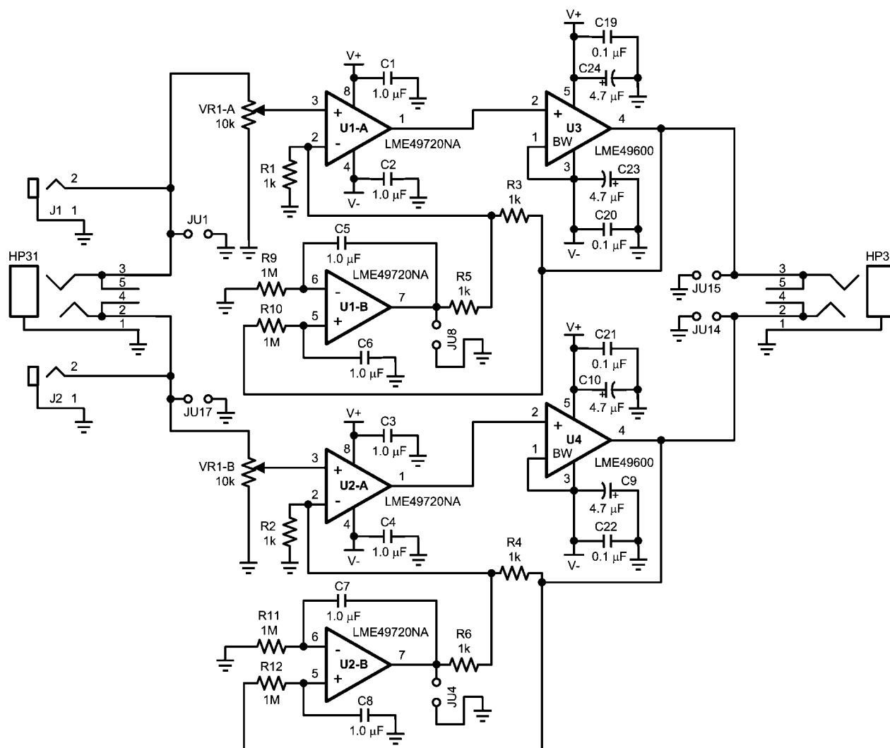
FIGURE 4. LME49600 delivers high output current for this high performance headphone amplifier
