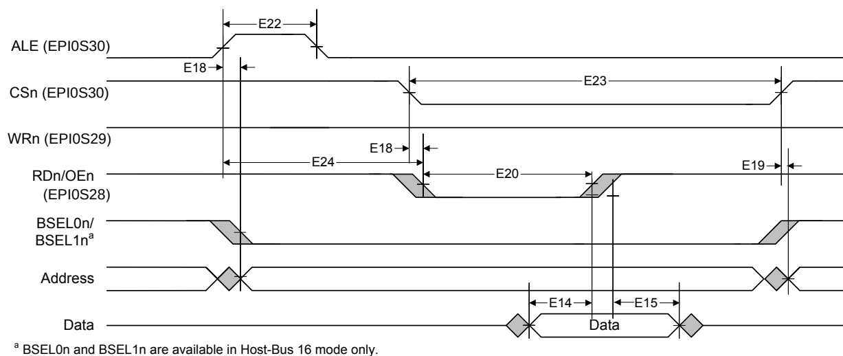
Figure 26-14. Host-Bus 8/16 Mode Read Timing
