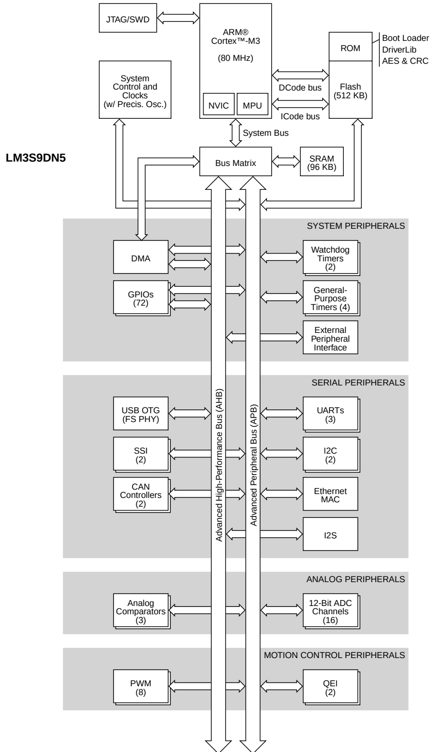
Figure 1-1. Stellaris LM3S9DN5 Microcontroller High-Level Block Diagram
