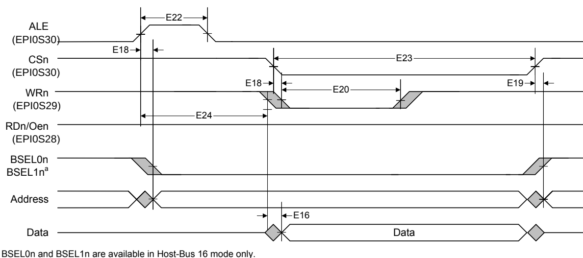
Figure 26-15. Host-Bus 8/16 Mode Write Timing
