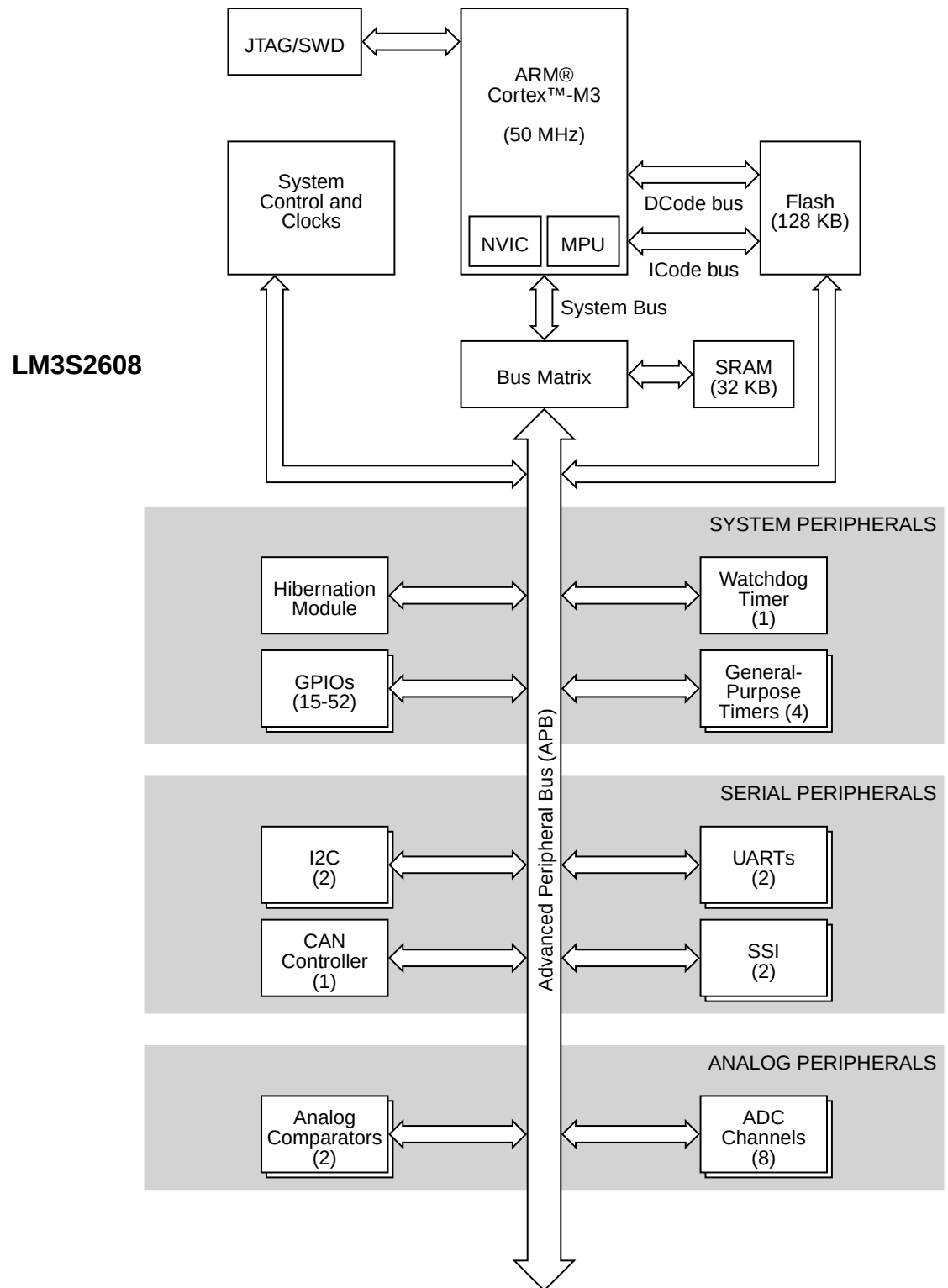
Figure 1-1. Stellaris LM3S2608 Microcontroller High-Level Block Diagram
