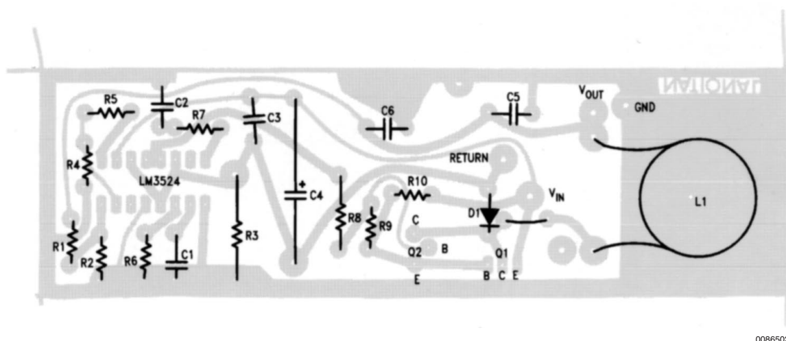
FIGURE 17. Stuffing Diagram, Component Side
