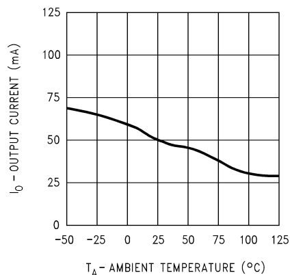
Reference Transistor Peak Output Current
