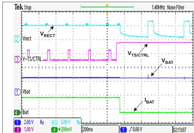
Figure 13. TS Fault
