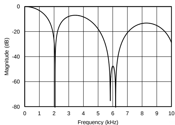
Figure 57. Filter Response (Data Rate = 2 kSPS)
