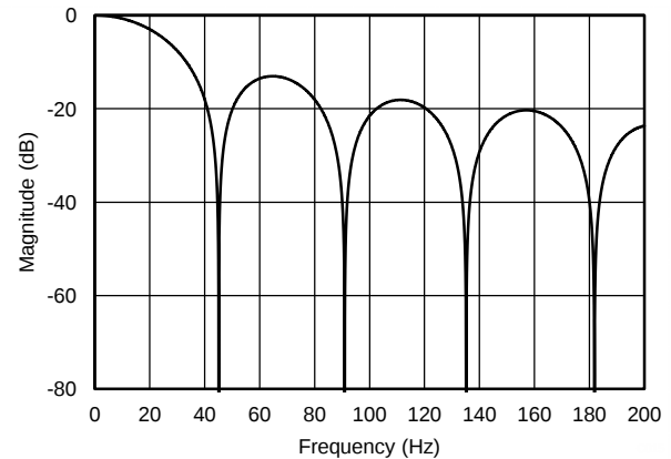
Figure 51. Filter Response (Data Rate = 45 SPS)
