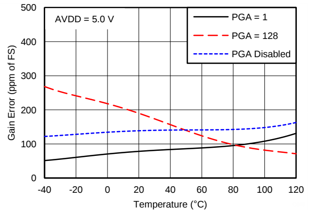
Figure 5. GAIN ERROR vs TEMPERATURE (AVDD = 5.0 V)
