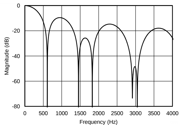
Figure 55. Filter Response (Data Rate = 600 SPS)
