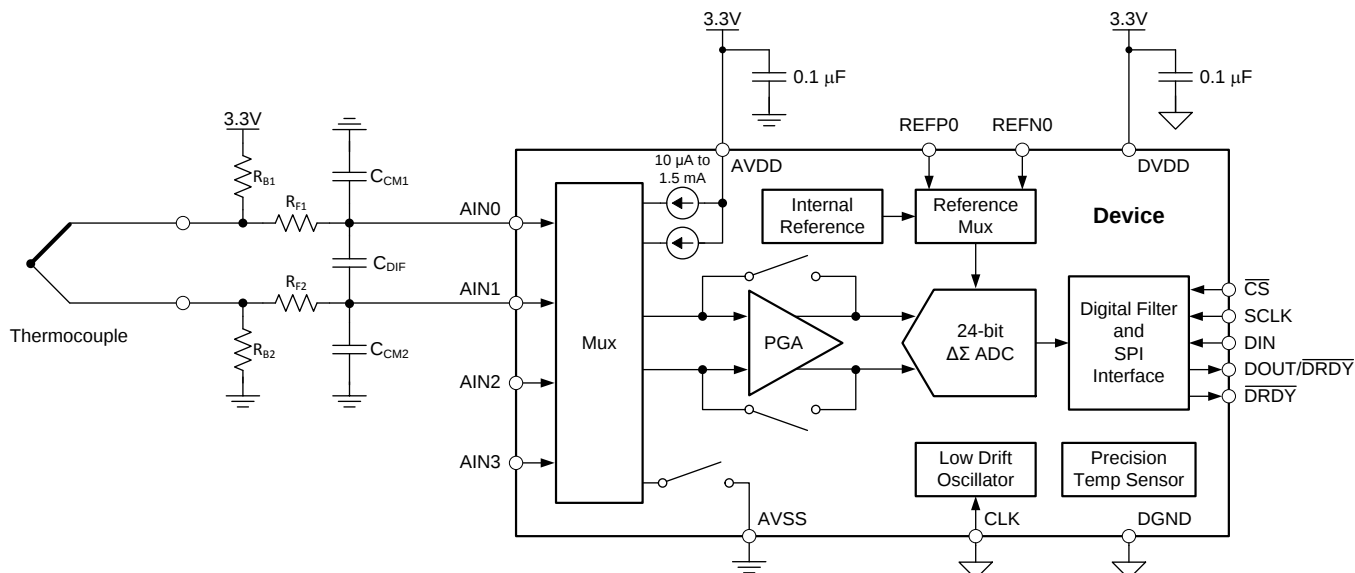
Figure 68. Thermocouple Measurement
