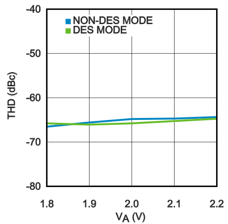
THD vs. SUPPLY VOLTAGE (ADC12D1600RF)
