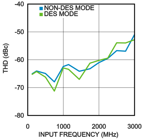
THD vs. INPUT FREQUENCY (ADC12D1600RF)
