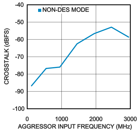
CROSSTALK vs. SOURCE FREQUENCY (ADC12D1000RF)
