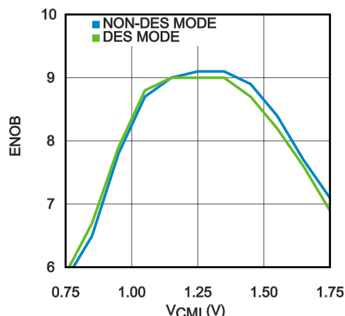
ENOB vs. V CM1 (ADC12D1600RF)
