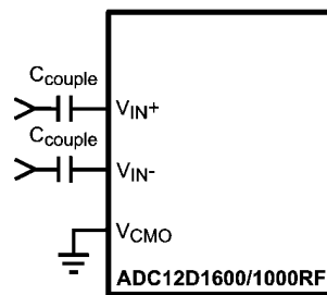
FIGURE 16. AC-coupled Differential Input
