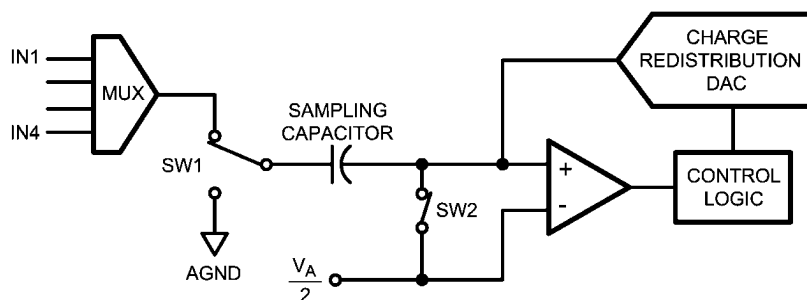
FIGURE 1. ADC124S051 in Track Mode
