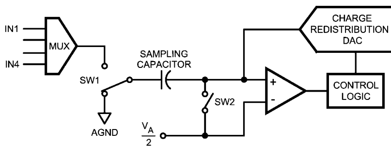
FIGURE 2. ADC124S051 in Hold Mode
