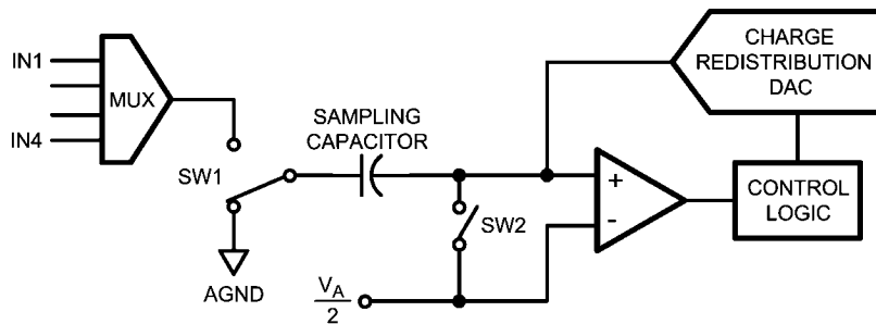
FIGURE 2. ADC104S021/ADC104S021Q in Hold Mode
