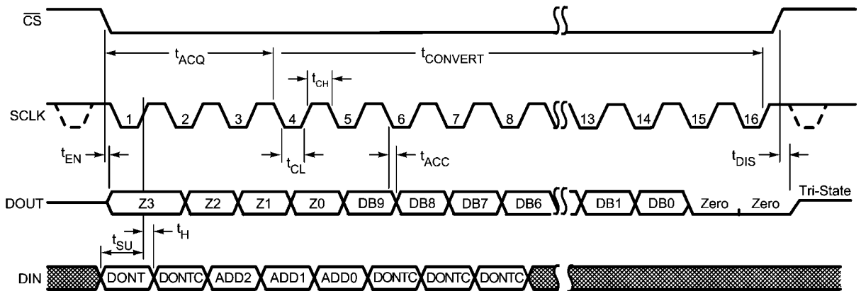
ADC104S021/ADC104S021Q Serial Timing Diagram
