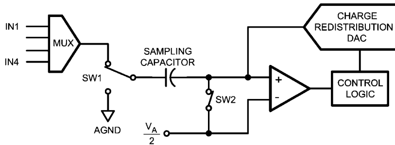
FIGURE 1. ADC104S021/ADC104S021Q in Track Mode
