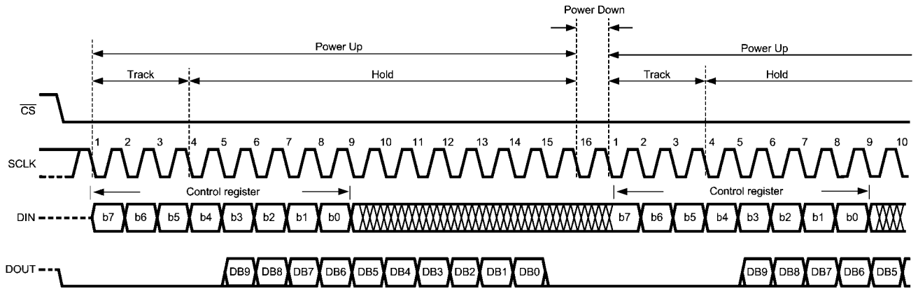
ADC104S021/ADC104S021Q Operational Timing Diagram
