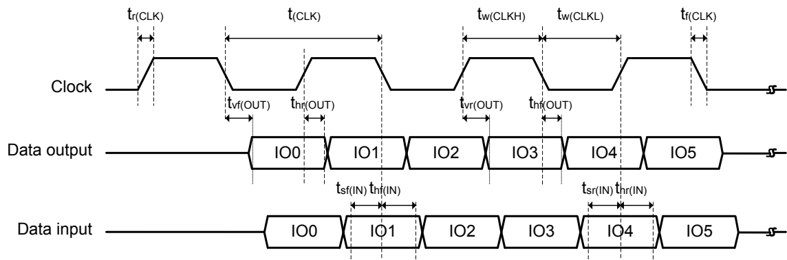
Figure 66. DDR mode
