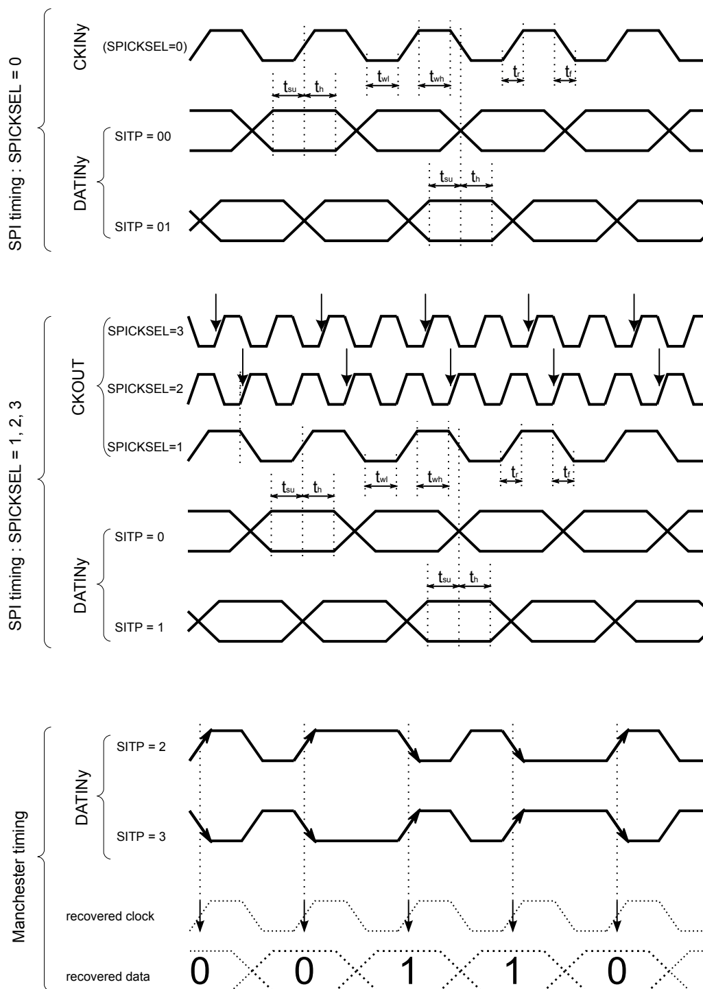
Figure 50. Channel transceiver timing diagrams
