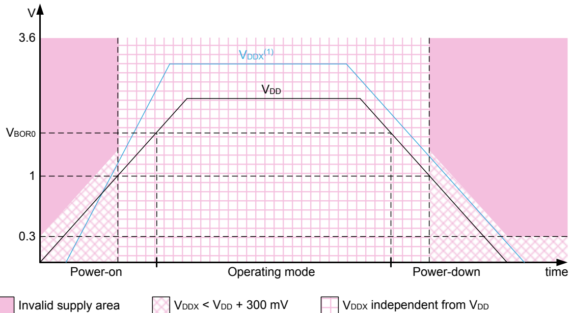
Figure 2. Power-up/power-down sequence
