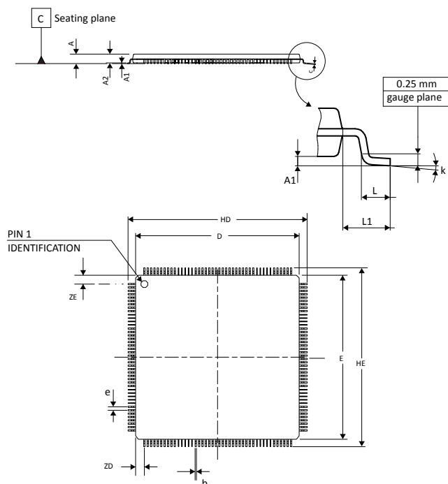
Figure 79. LQFP - 176 pins, 24 x 24 mm low profile quad flat package outline
