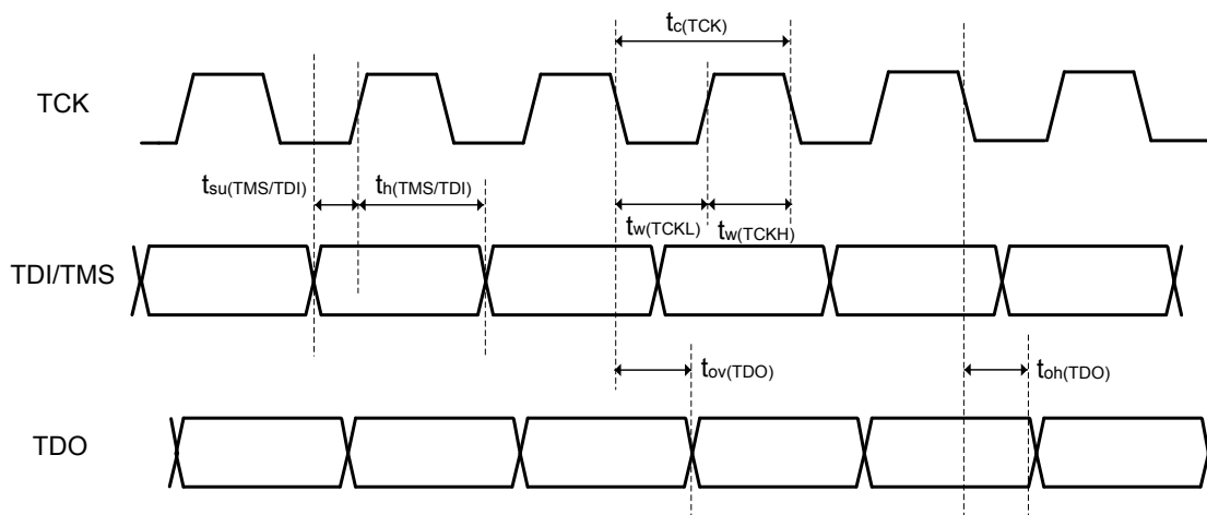
Figure 68. JTAG timing diagram
