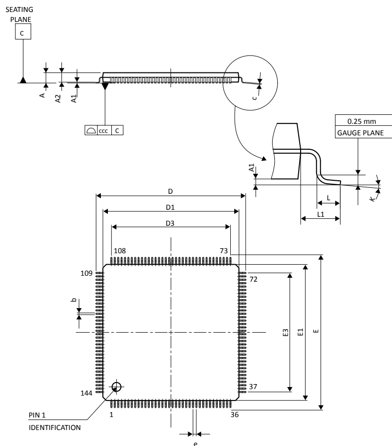
Figure 76. LQFP - 144 pins, 20 x 20 mm low-profile quad flat package outline
