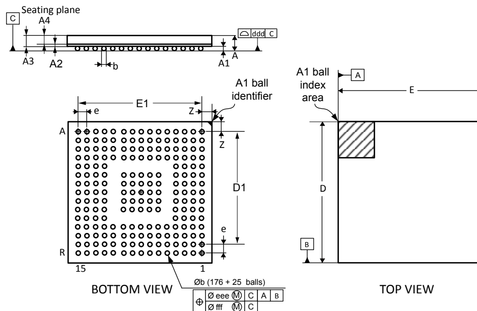
Figure 85. UFPGA - 176+25 balls, 10 x 10 mm, 0.65 mm pitch, ultra fine pitch ball grid array package outline
