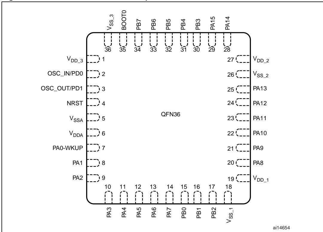
Figure 6. STM32F103xx VFQFPN36 pinout
