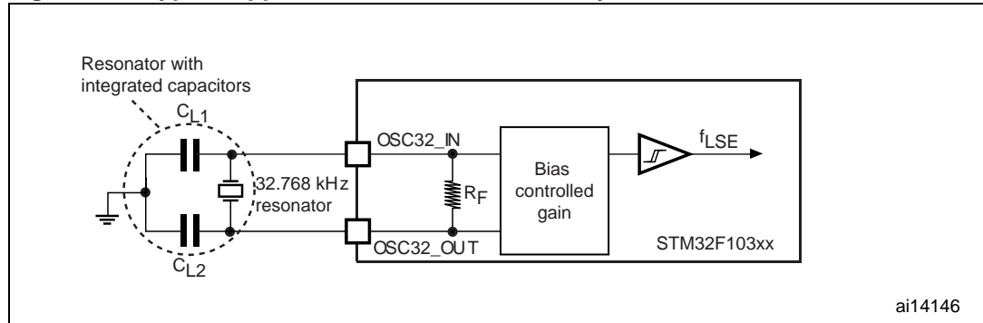
Figure 20. Typical application with a 32.768 kHz crystal
