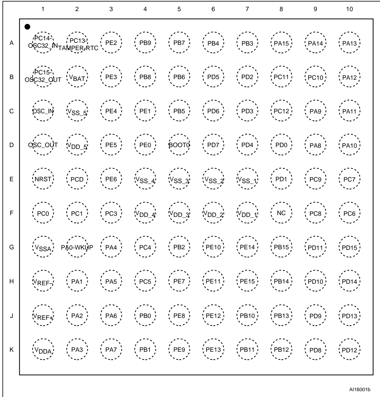
Figure 2. STM32F103xx performance line BGA100 ballout
