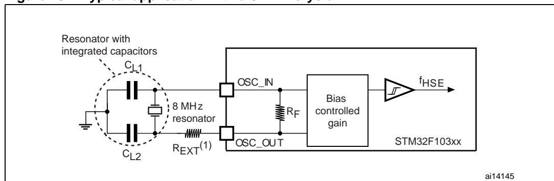
Figure 19. Typical application with a 8-MHz crystal
