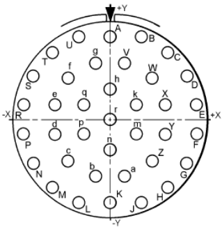
Contact Layout
