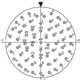
Contact Layout
