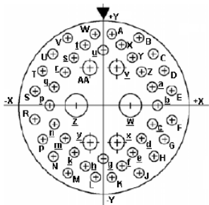
Contact Layout
