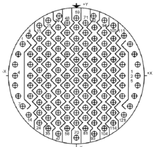
Contact Layout
