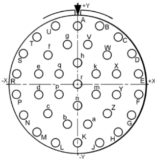
Contact Layout
