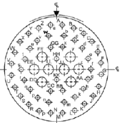
Contact Layout
