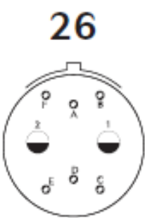
Contact Layout
