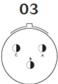
Contact Layout
