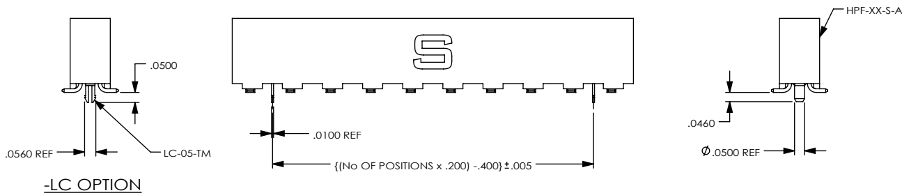
FIG 2 -LC & -A OPTIONS (-LC & -A OPTION ONLY AVAILABLE ON -02 LEAD STYLE) (SAME AS FIG 1 EXCEPT WHERE SHOWN)
