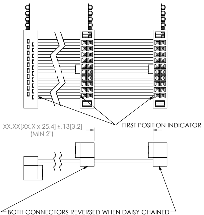
FIG. 6 (FFSD-10-D-XX.XX-01-X-N-DXX-R SHOWN) (SAME AS FIG. 1, DIFFERENT AS SHOWN) (NOT AVAILABLE WITH -RN1 OR -RN2 OPTION) (2.00[50.8] MINIMUM, 1.00[25.4] INCREMENTS)
