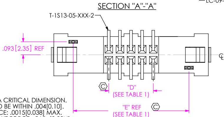
FIG 1 (EHT-105-01-XX-D-SM-SR-LC SHOWN)
