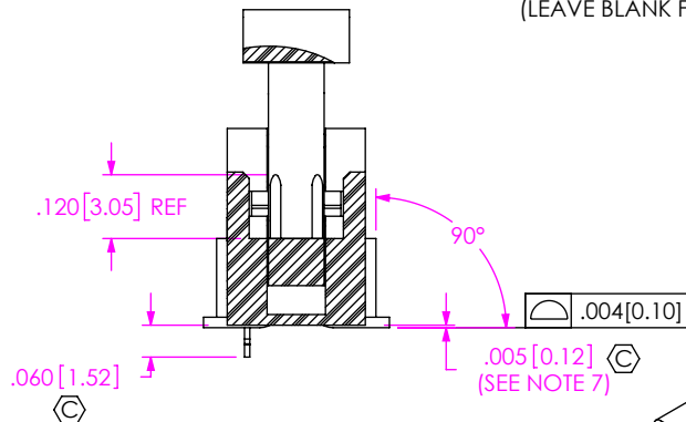
FIG 1 (EHT-105-01-XX-D-SM-SR-LC SHOWN)
