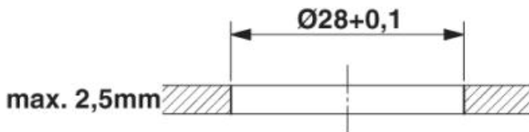
Dimensional drawing
