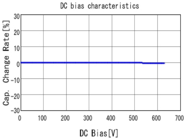
■ GRM31C5C2J472JWA3 C-DC bias capchange, 25.0degC, AC1V
