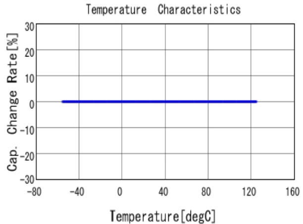
■ GRM31C5C2J472JWA3 C-Temp. capchange, DC0V, AC1Vrms
