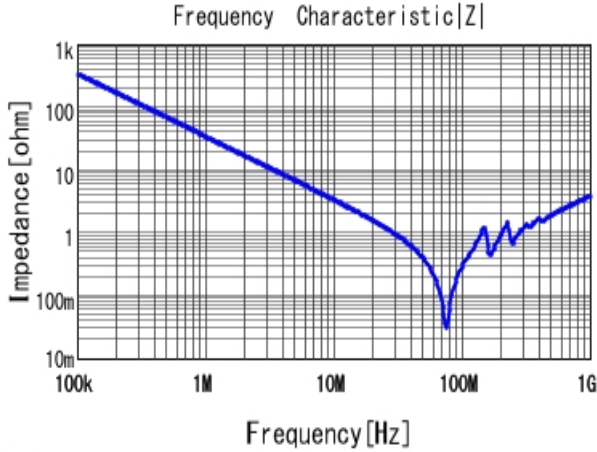
■ GRM31C5C2J472JWA3 |Z| DC0V, 25degC
