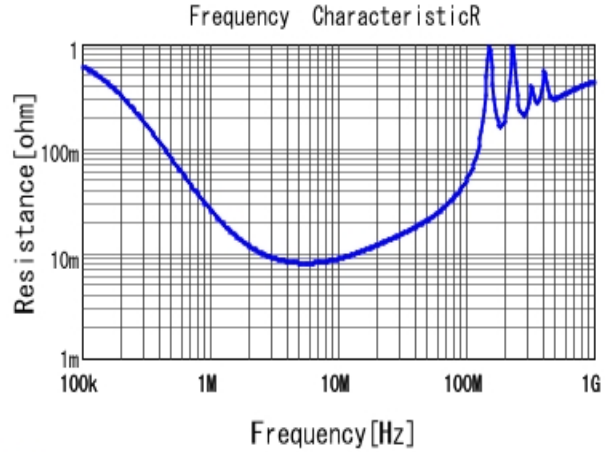
■ GRM31C5C2J472JWA3 R DC0V, 25degC
