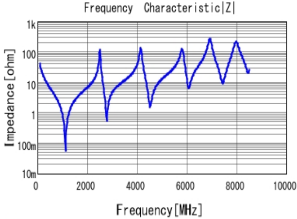
■ GQM22M5C2H390GB01 |Z| DC0V, 25degC
