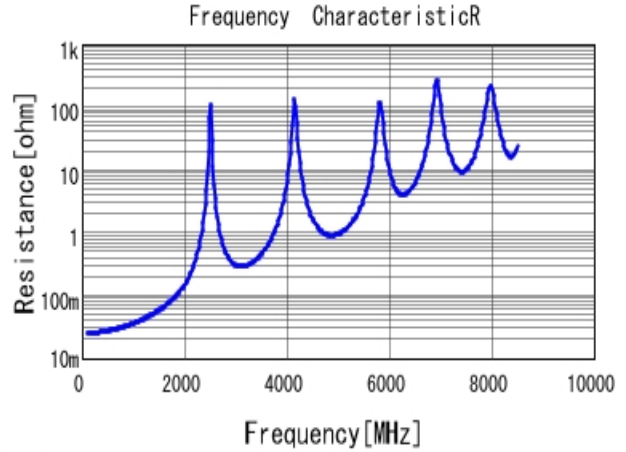
■ GQM22M5C2H390GB01 R DC0V, 25degC
