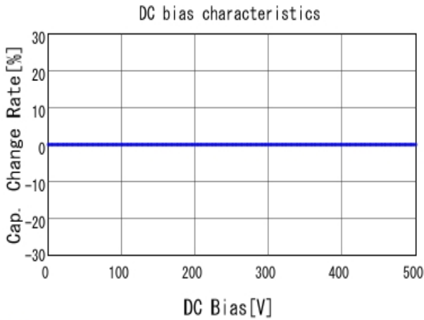
■ GQM22M5C2H390GB01 C-DC bias capchange, 25.0degC, AC1V
