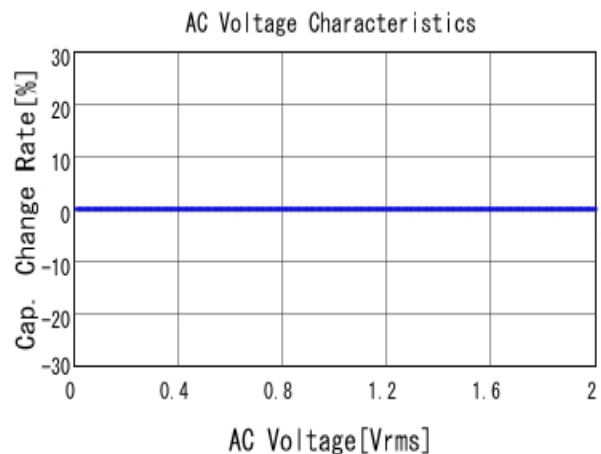
■ GQM1555C2D1R2BB01 C-AC Voltage capchange, DC0V, 25.0d
