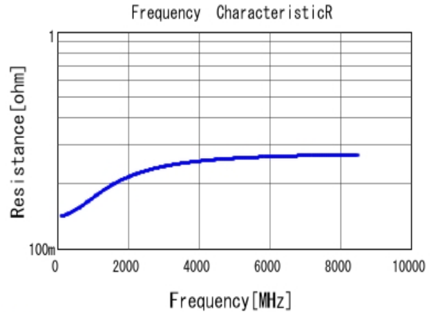
■ GQM1555C2D1R2BB01 R DC0V, 25degC
