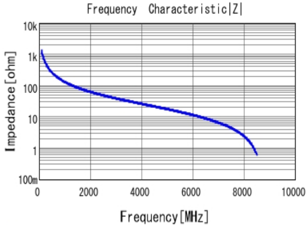
■ GQM1555C2D1R2BB01 |Z| DC0V, 25degC
