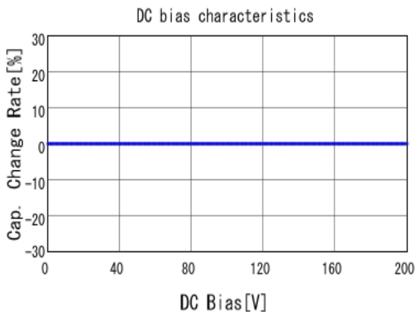
■ GQM1555C2D1R2BB01 C-DC bias capchange, 25.0degC, AC1V
