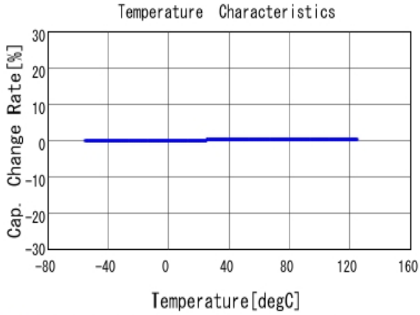
■ GJM1555C1H8R5WB01 C-Temp. capchange, DCOV, AC1Vrms
