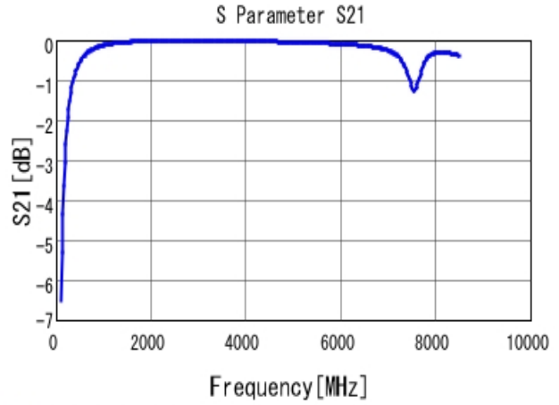
■ GJM1555C1H8R5WB01 S21 DCOV, 25degC
