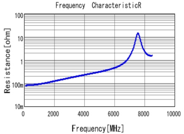
■ GJM1555C1H8R5WB01 R DC0V, 25degC
