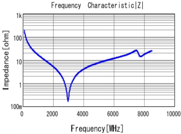
■ GJM1555C1H8R5WB01 |Z| DC0V, 25degC
