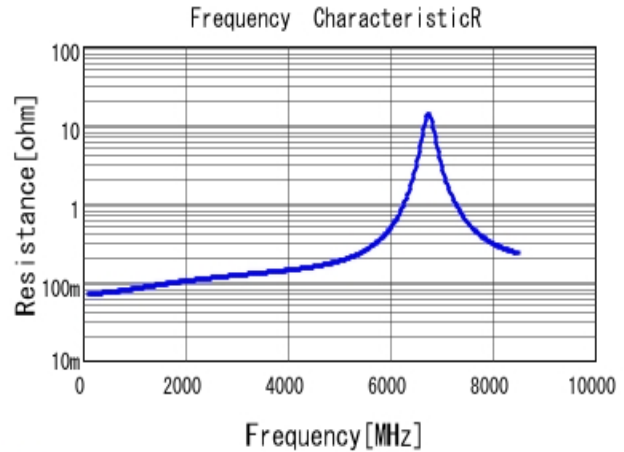
■ GCQ1555C1H9R8DB01 R DC0V, 25degC
