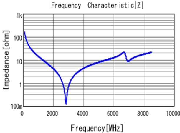
■ GCQ1555C1H9R8DB01 |Z| DC0V, 25degC
