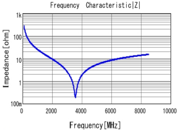
■ GCQ1555C1H5R8CB01 |Z| DC0V, 25degC
