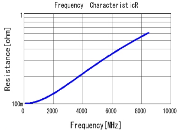
■ GCQ1555C1H5R8CB01 R DC0V, 25degC
