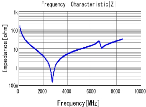
■ GCQ1555C1H100FB01 |Z| DC0V, 25degC
