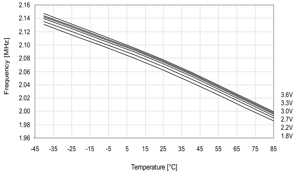
Figure 33-147. 2MHz internal oscillator frequency vs. temperature.
