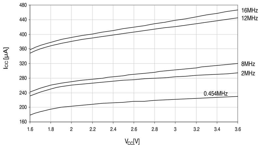
Figure 33-20. Standby supply current vs. V_{CC} .
