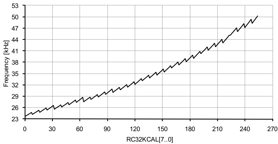
Figure 33-227. 32.768kHz internal oscillator frequency vs. calibration value.
