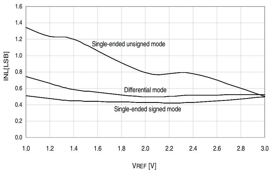
Figure 33-36. INL error vs. external V_{REF} .
