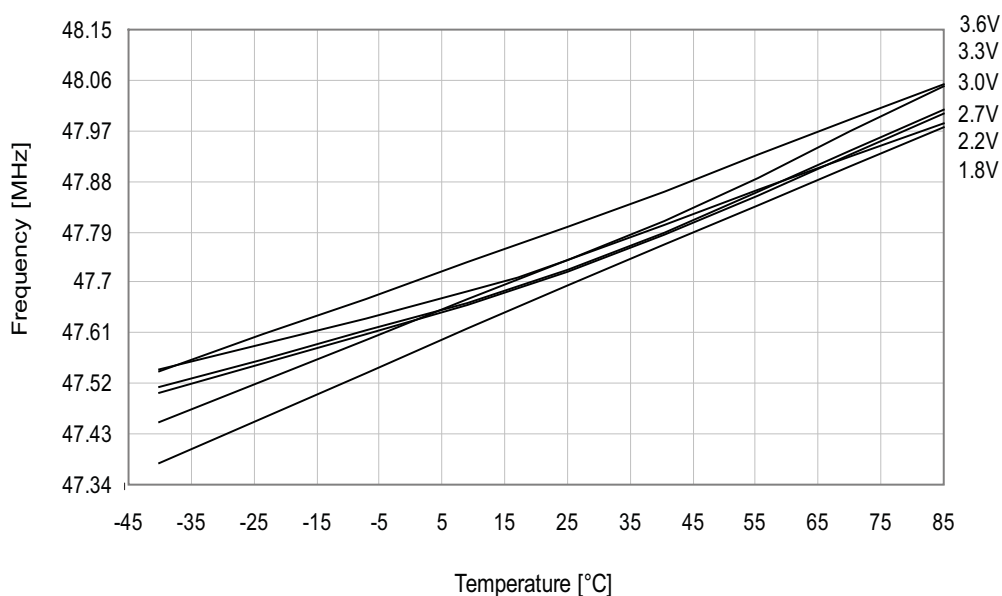
Figure 33-154. 48MHz internal oscillator frequency vs. temperature. DPLL enabled, from the 32.768kHz internal oscillator.
