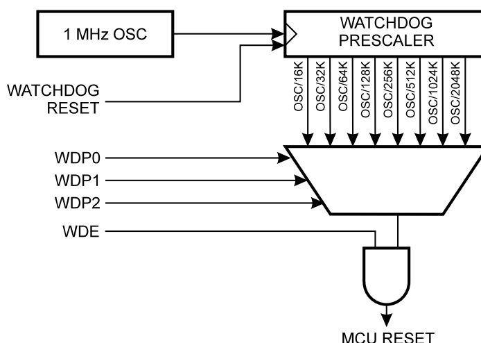
Figure 20. Watchdog Timer
