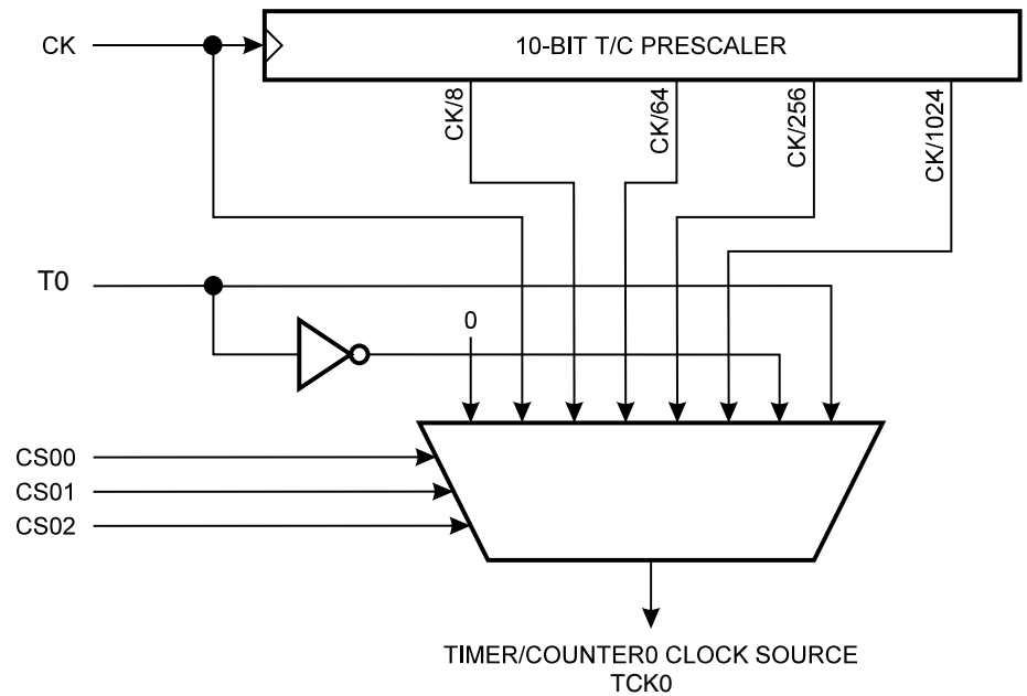
Figure 18. Timer/Counter0 Prescaler
