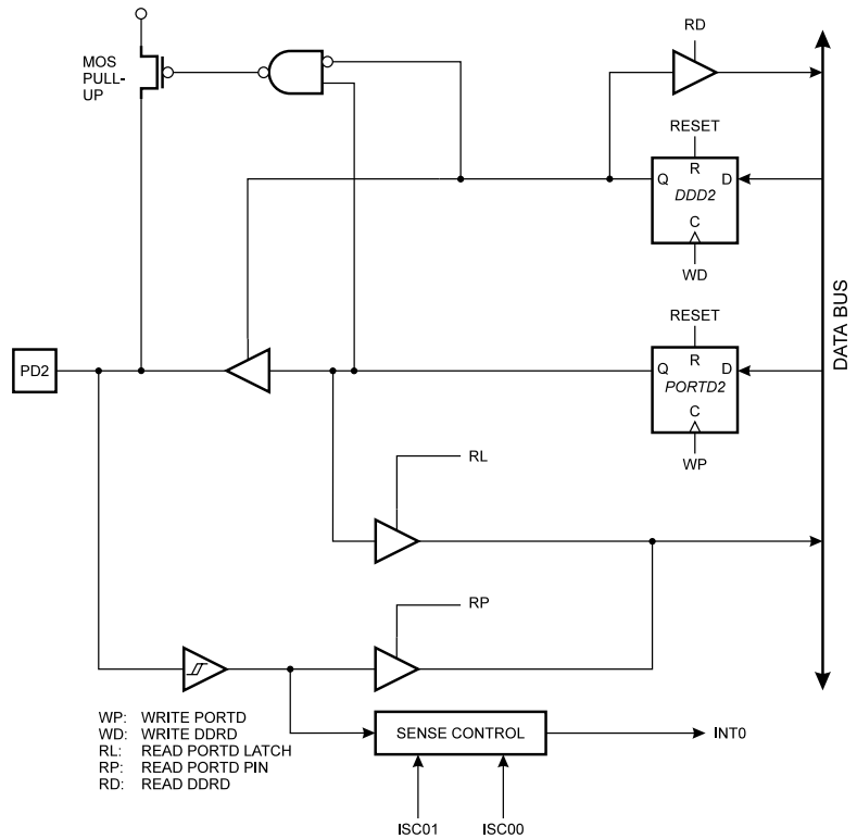
Figure 28. Port D Schematic Diagram (Pin PD2)
