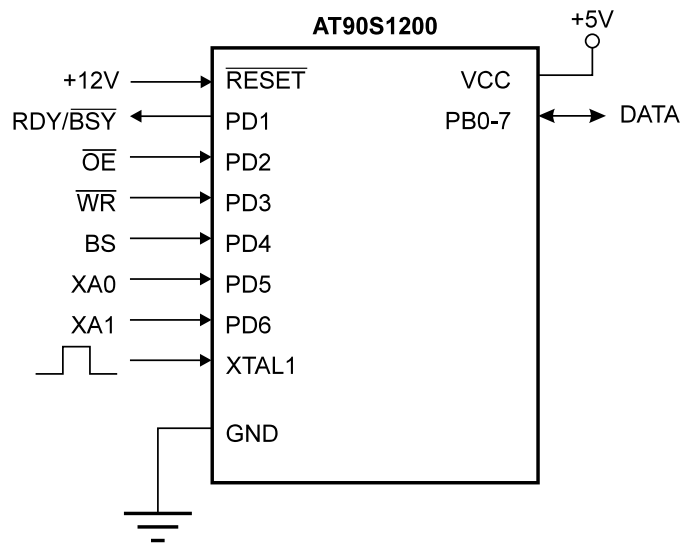
Figure 30. Parallel Programming
