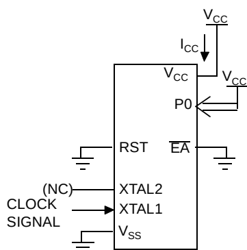
Figure 80. I_{CC} Test Condition, Power-Down Mode
