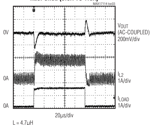
STEP-DOWN REGULATOR LOAD-TRANSIENT RESPONSE (0.3A TO 1.8A)
