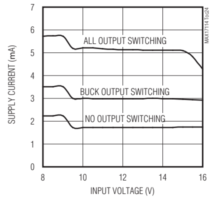
INVL SUPPLY CURRENT vs. INPUT VOLTAGE
