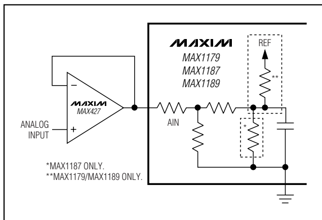
Figure 11. MAX1179/MAX1187/MAX1189 Fast-Settling Input Buffer
