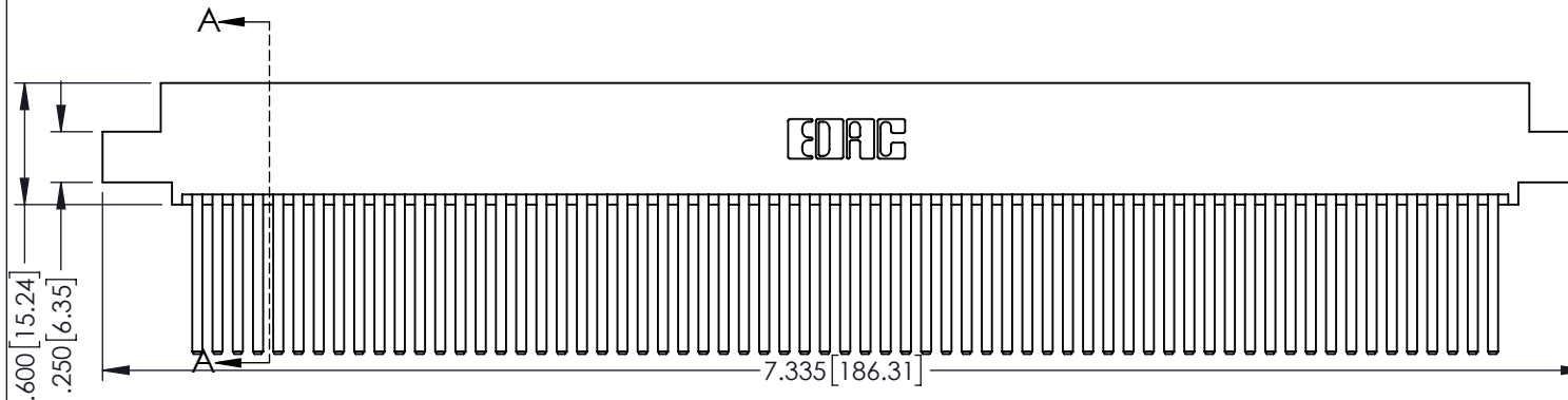
345/395 SERIES CARD EDGE CONNECTOR PART NUMBER: 345-130-544-504
