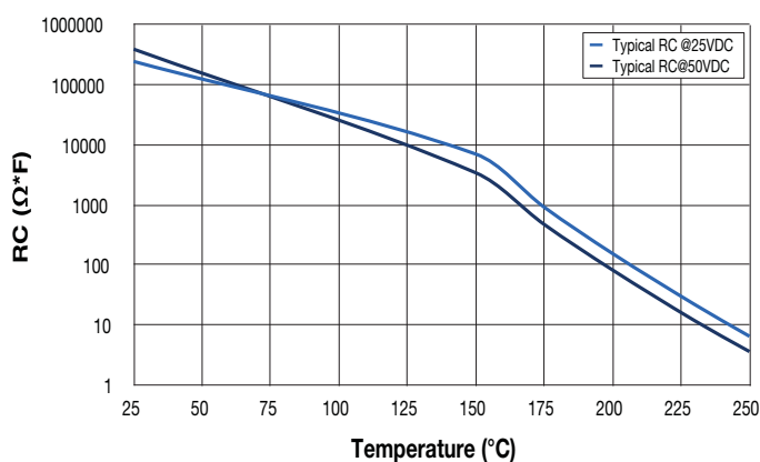
RC vs Temperature (C0G Dielectric)
