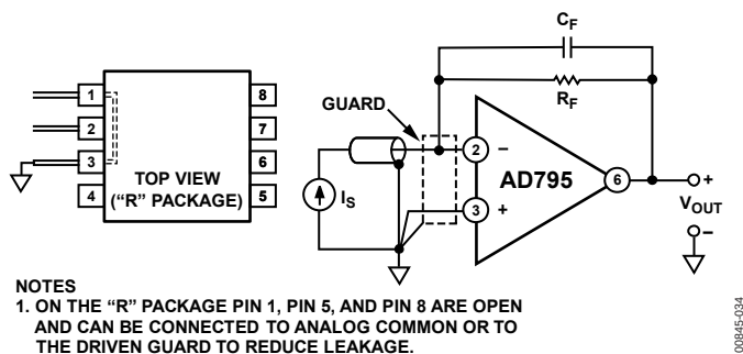
Figure 34. Guarding Scheme—Inverter
