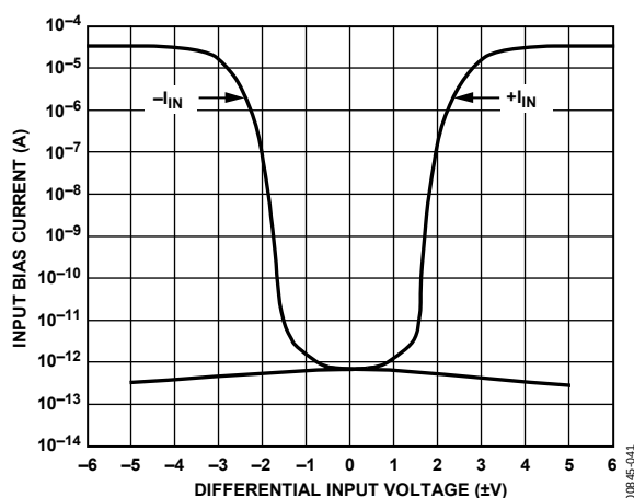
Figure 41. Input Bias Current vs. Differential Input Voltage
