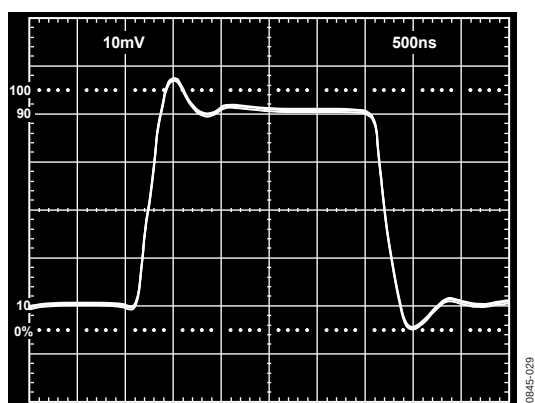
Figure 29. Unity Gain Inverter Small Signal Pulse Response
