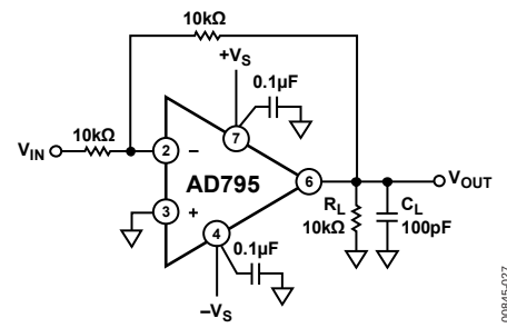
Figure 27. Unity Gain Inverter
