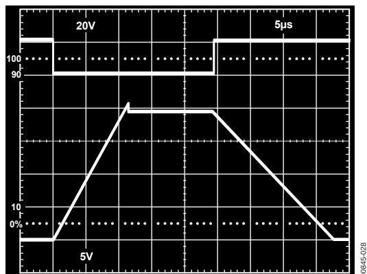
Figure 28. Unity Gain Inverter Large Signal Pulse Response
