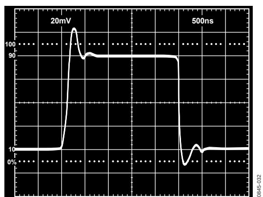
Figure 32. Unity Gain Follower Small Signal Pulse Response
