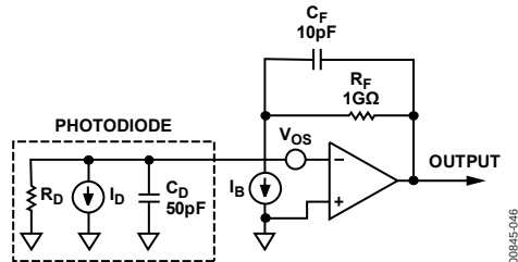
Figure 46. A Photodiode Model Showing DC Error Sources
