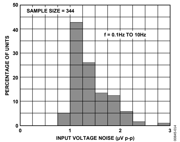
Figure 14. Typical Distribution of Input Voltage Noise
