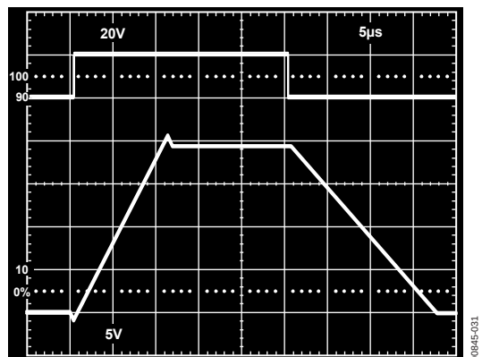
Figure 31. Unity Gain Follower Large Signal Pulse Response
