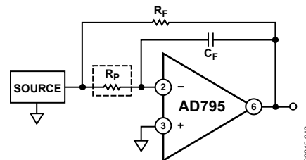
Figure 42. Inverter with Input Current Limit
