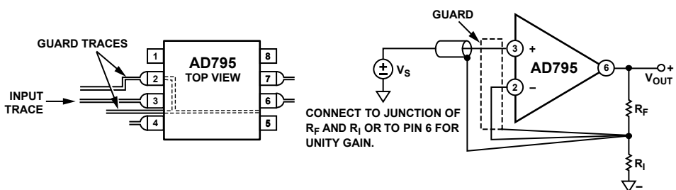
Figure 35. Guard Scheme—Follower
