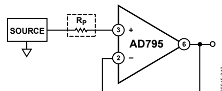
Figure 43. Follower with Input Current Limit
