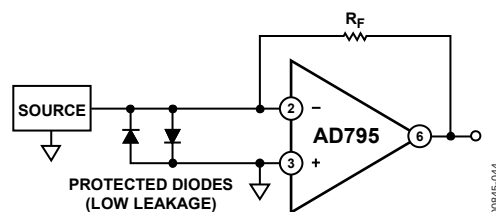
Figure 44. Input Voltage Clamp with Diodes
